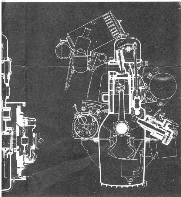
ings show the general arrangement of the TC engine, which has the highly creditable output of 45 b.h.p. per litre and 2.5 square inch of piston area.
