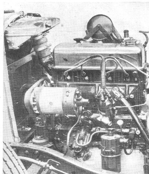
er," shows how the engine is set well back in the frame, the latter being stiffened amidships. This latter carries toolbags and accumulators. The well-raked steering column carries a large column length. (Right) The near side of the engine. The large capacity dynamo has constant- which receives oil through a floating pick-up, delivers to an external full-flow filter.
